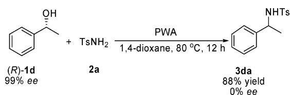
Scheme 1. Amidation reaction of ( R )- 1d with 2a .
